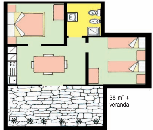
THREE-ROOMS TERRACED HOUSE - 4/5 PEOPLE
